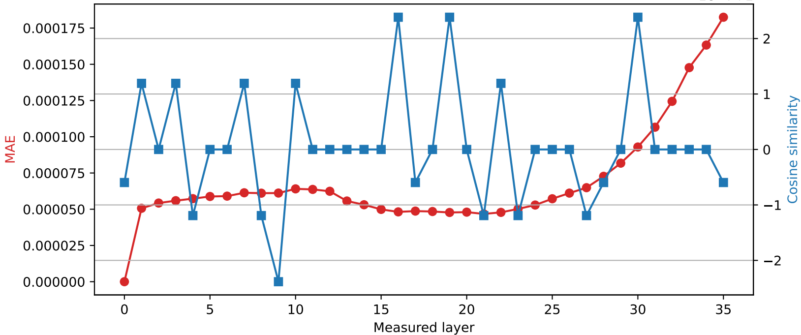
Qwen2.5-3B | Quantized layer 0 | float32 \rightarrow int16
