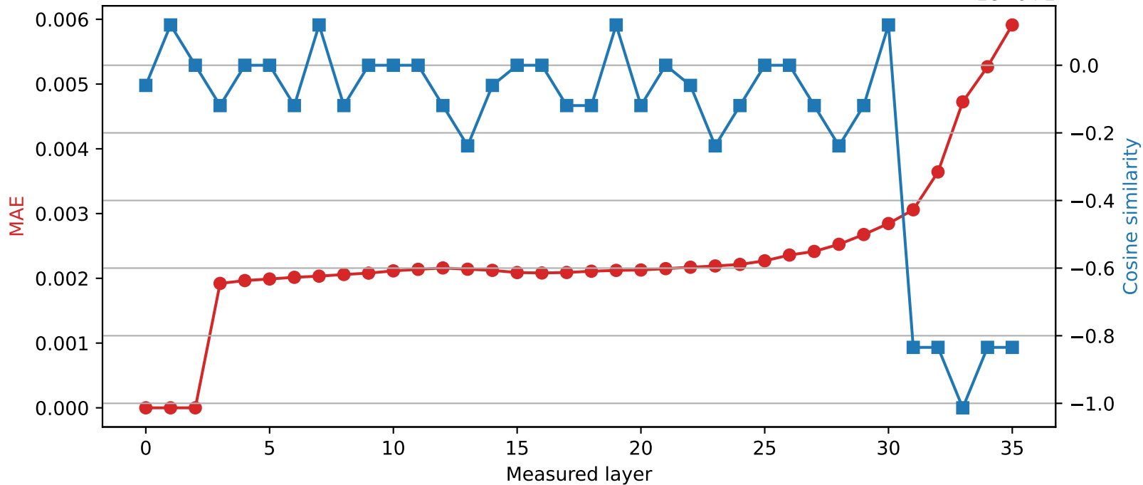
Qwen2.5-3B | Quantized layer 2 | float32 → int16
