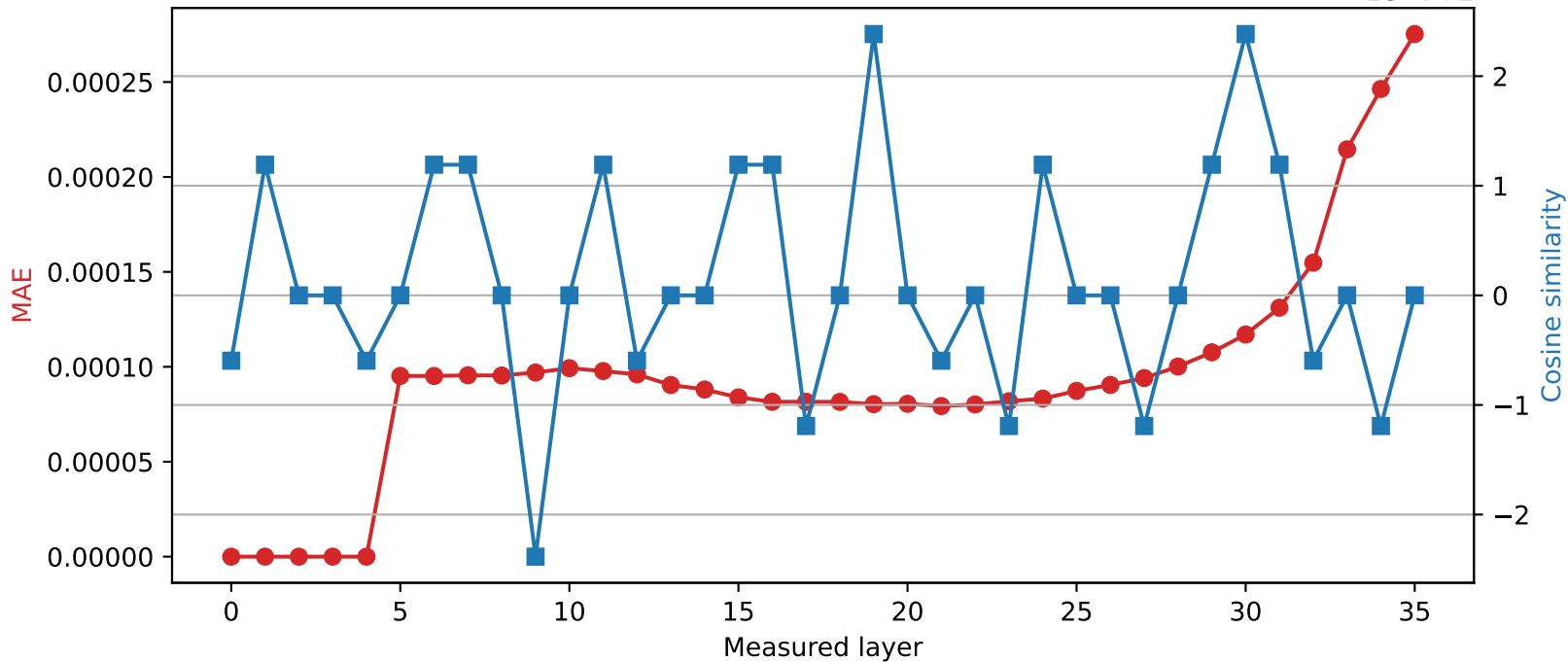
Qwen2.5-3B | Quantized layer 4 | float32 → int16
