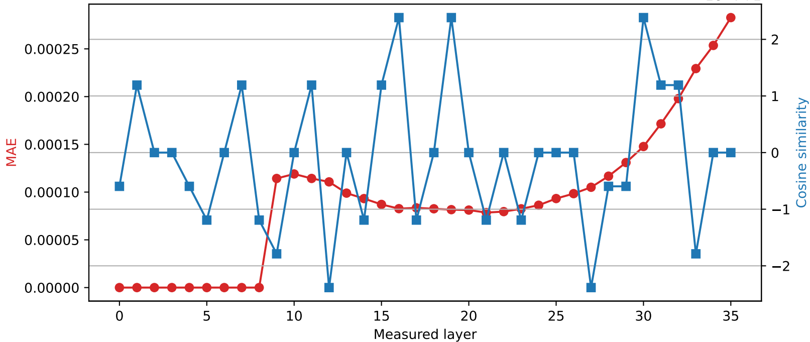
Qwen2.5-3B | Quantized layer 8 | float32 → int16
