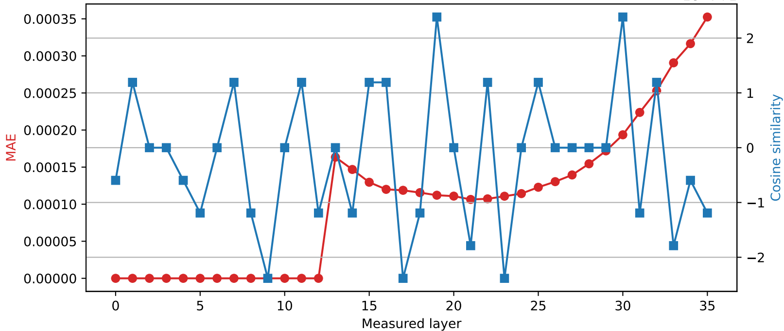
Qwen2.5-3B | Quantized layer 12 | float32 → int16
