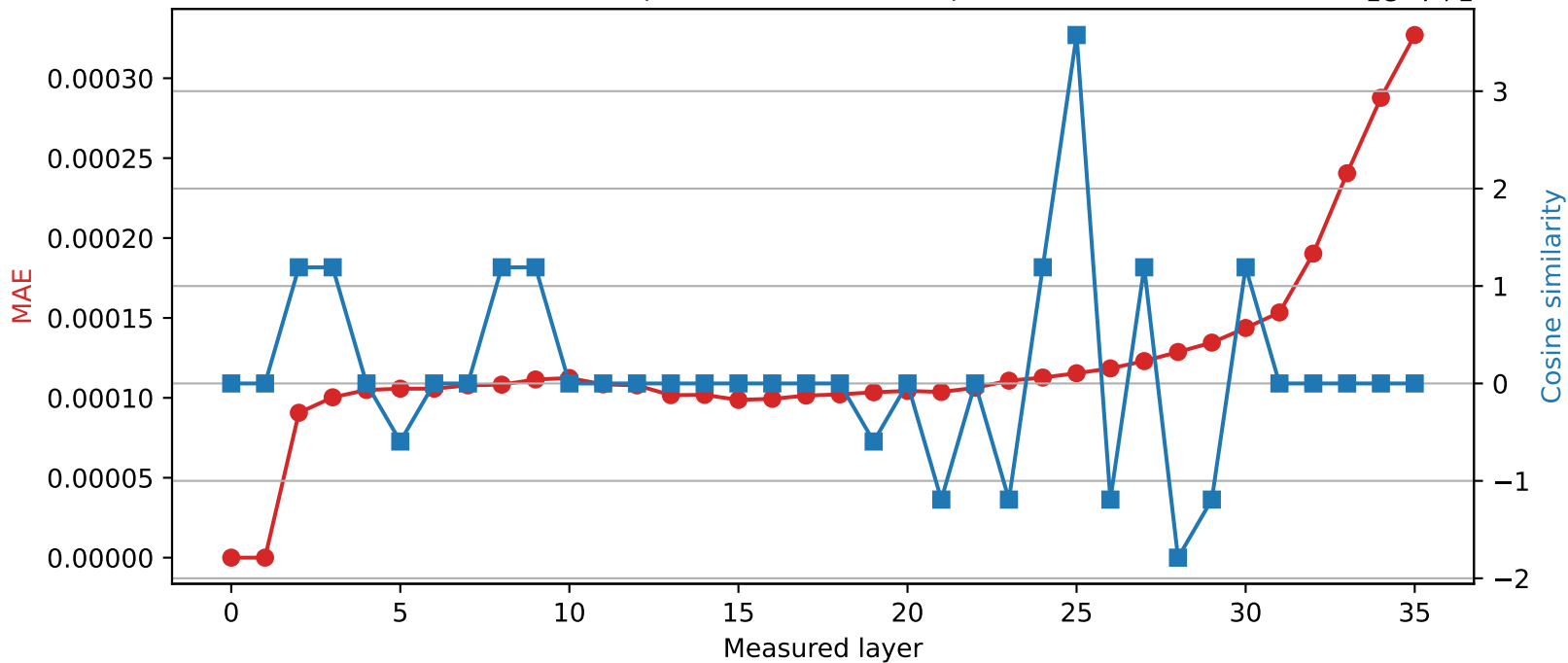
Qwen2.5-3B | Quantized layer 1 | float32 \rightarrow int16
