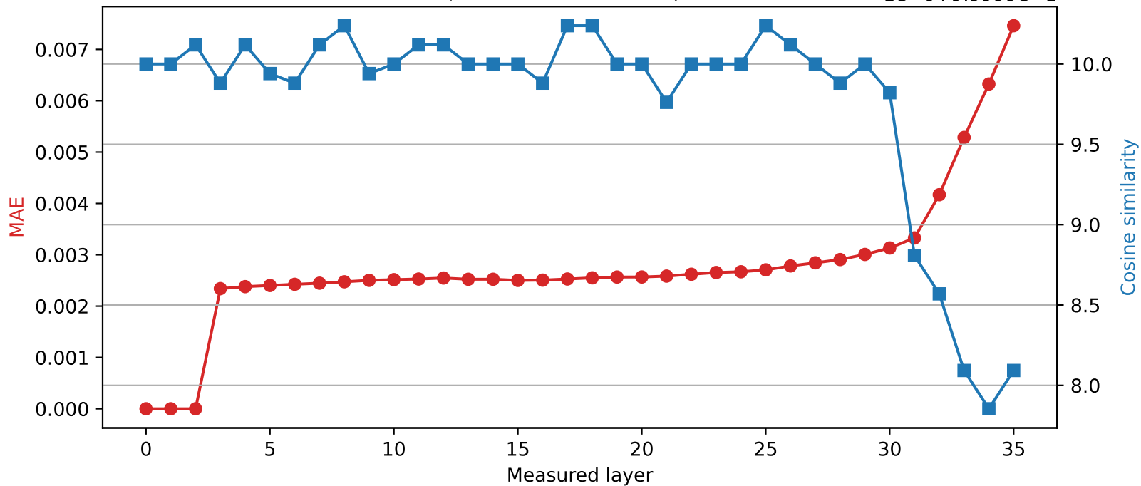
Qwen2.5-3B | Quantized layer 2 | float32 \rightarrow int16
