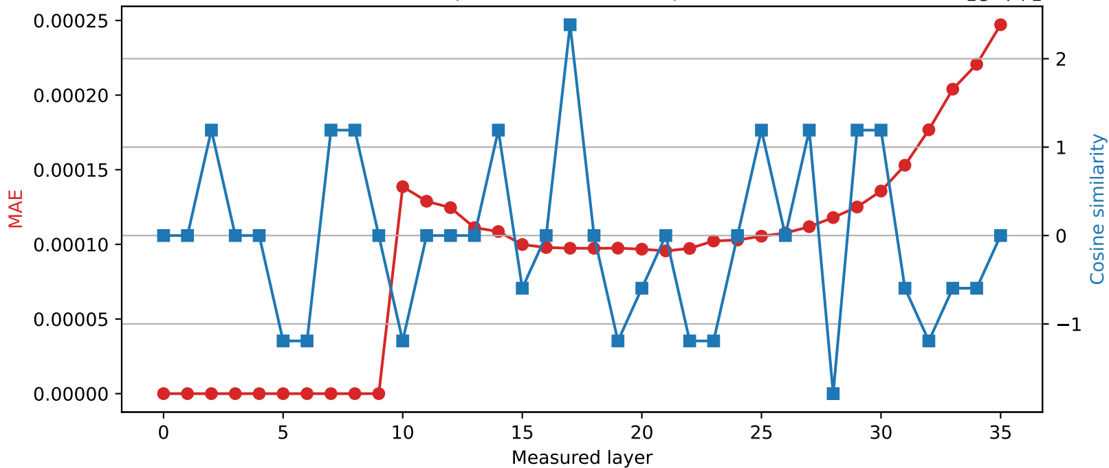
Qwen2.5-3B | Quantized layer 9 | float32 → int16
