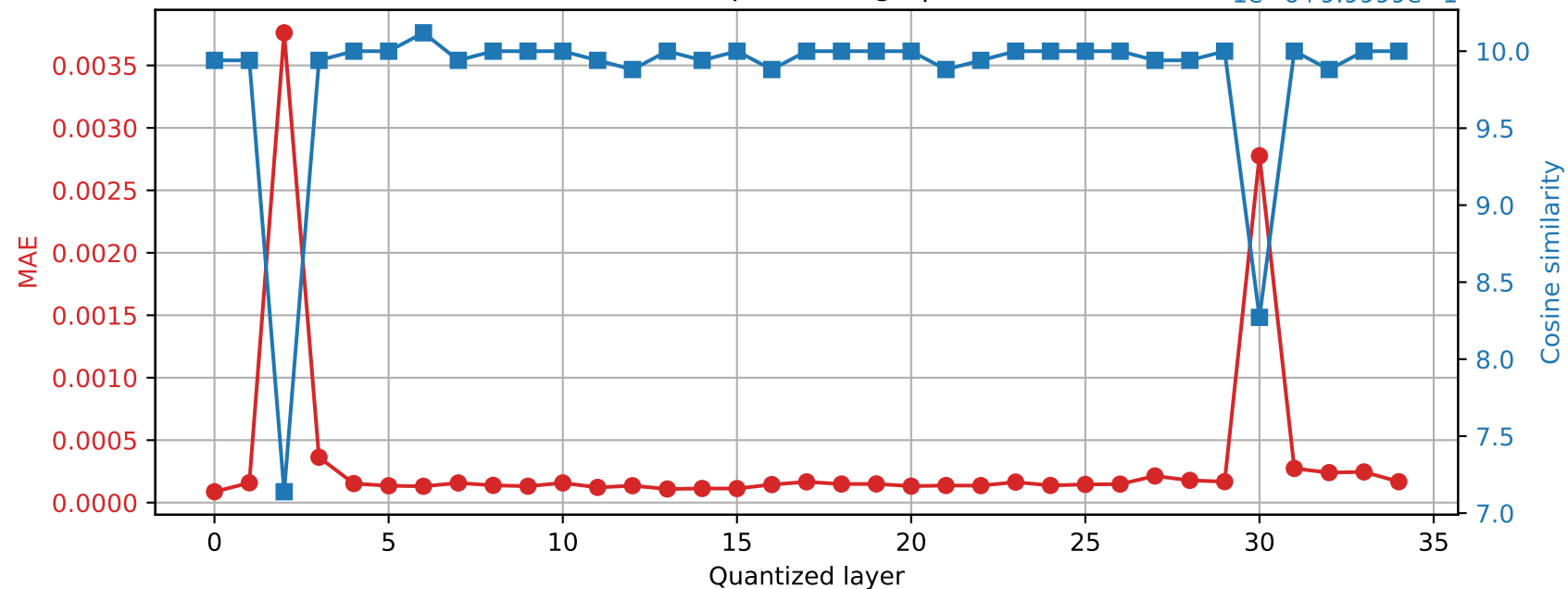
Qwen2.5-3B | Prompt 3 Final RMSNorm output damage | float32 \rightarrow int16
