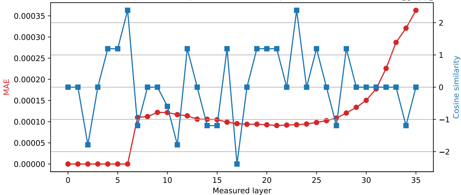
Qwen2.5-3B | Quantized layer 6 | float32 \rightarrow int16
