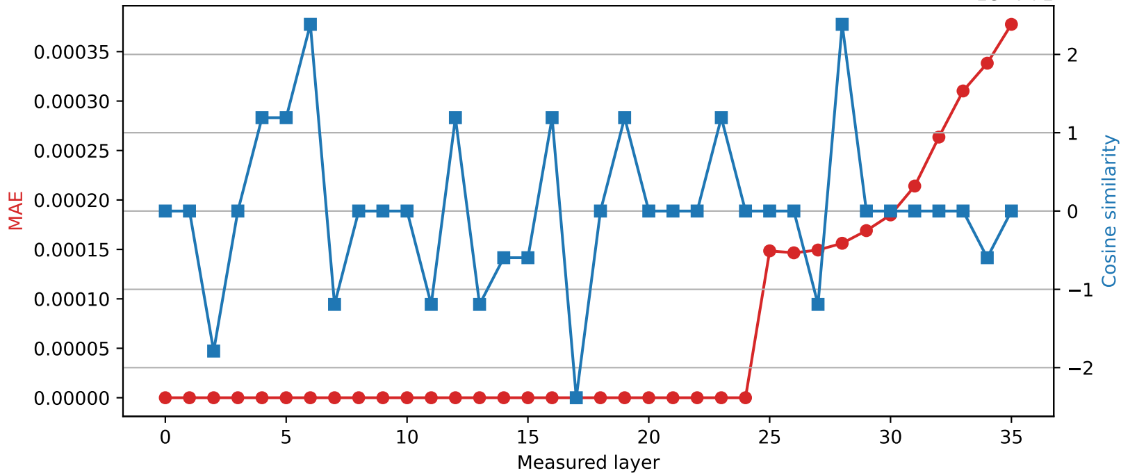
Qwen2.5-3B | Quantized layer 24 | float32 \rightarrow int16
