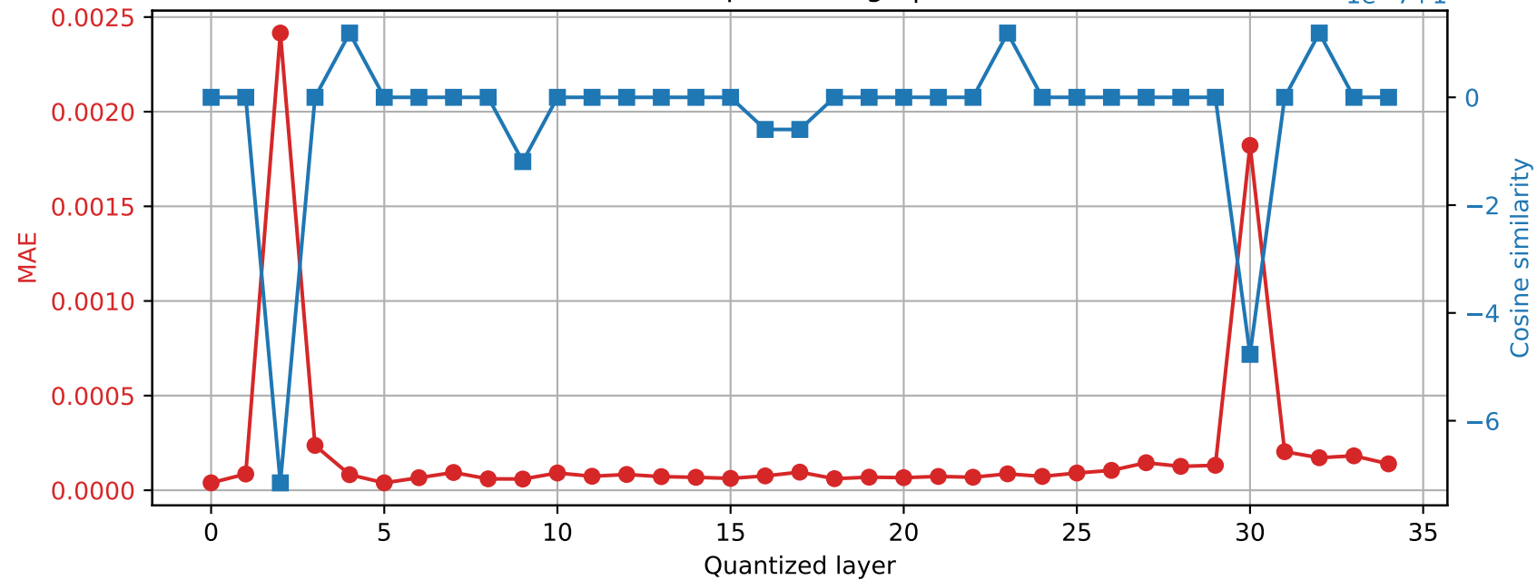
Qwen2.5-3B | Prompt 4 Final RMSNorm output damage | float32 → int16
