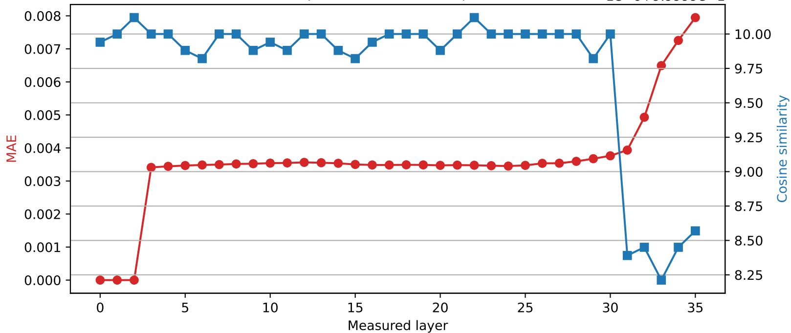
Qwen2.5-3B | Quantized layer 2 | float32 → int16 1e-6+9.9999e-1
