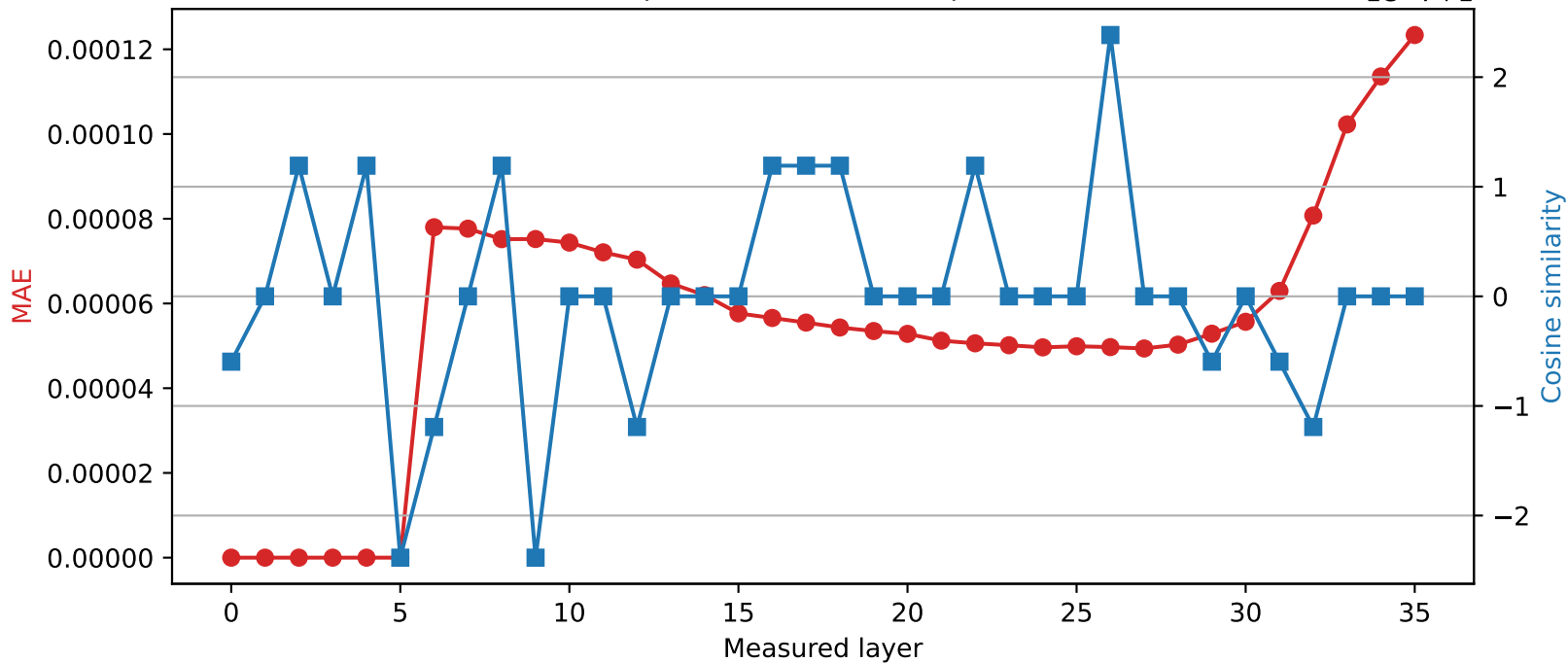
Qwen2.5-3B | Quantized layer 5 | float32 \rightarrow int16
