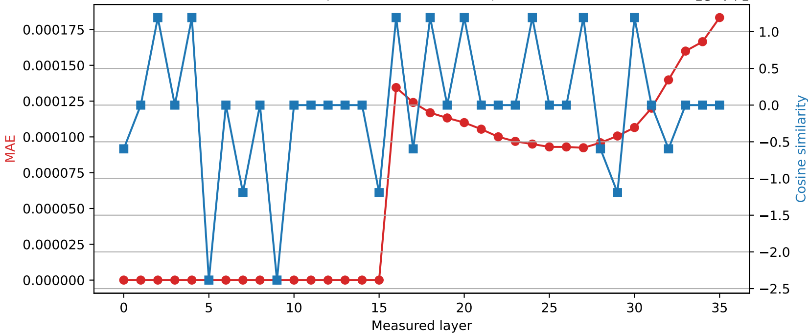
Qwen2.5-3B | Quantized layer 15 | float32 \rightarrow int16
