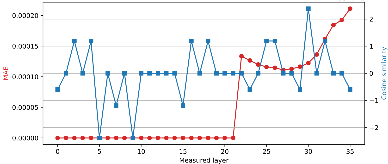
Qwen2.5-3B | Quantized layer 21 | float32 → int16
