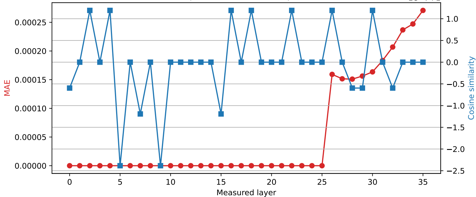
Qwen2.5-3B | Quantized layer 25 | float32 \rightarrow int16
