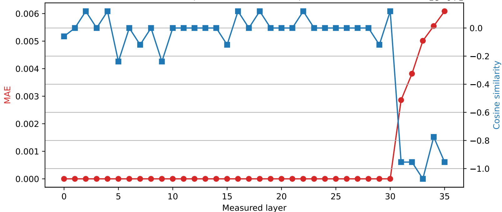
Qwen2.5-3B | Quantized layer 30 | float32 \rightarrow int16
