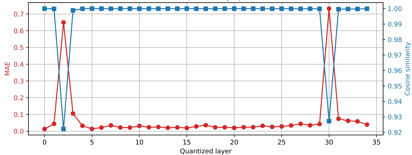
Qwen2.5-3B | Prompt 0 Final RMSNorm output damage | float32 \rightarrow int8
