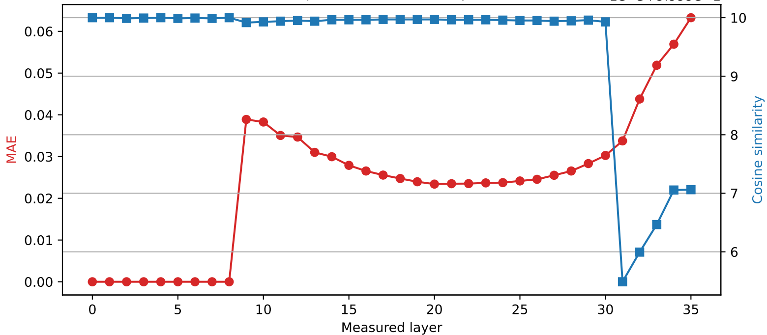
Qwen2.5-3B | Quantized layer 8 | float32 → int8
