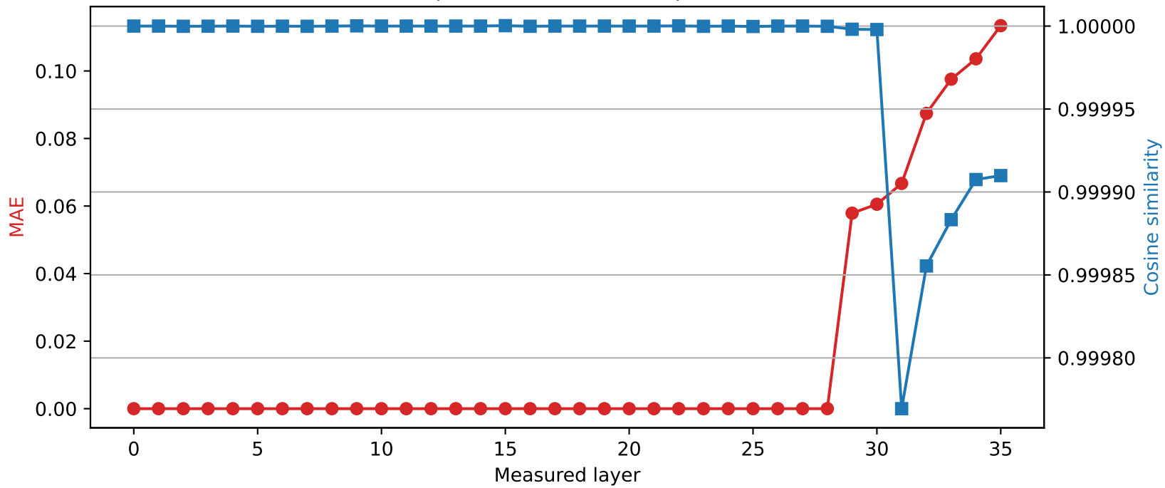
Qwen2.5-3B | Quantized layer 28 | float32 \rightarrow int8
