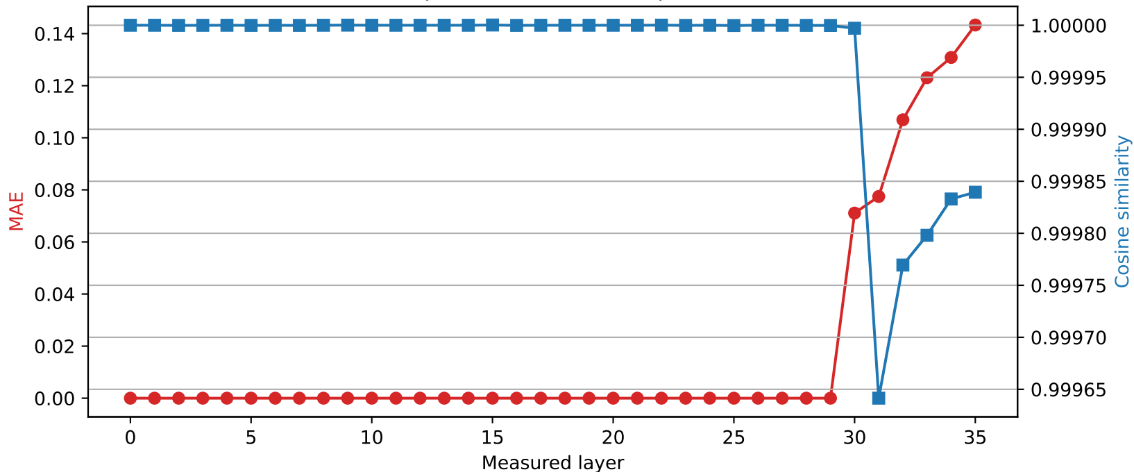
Qwen2.5-3B | Quantized layer 29 | float32 → int8
