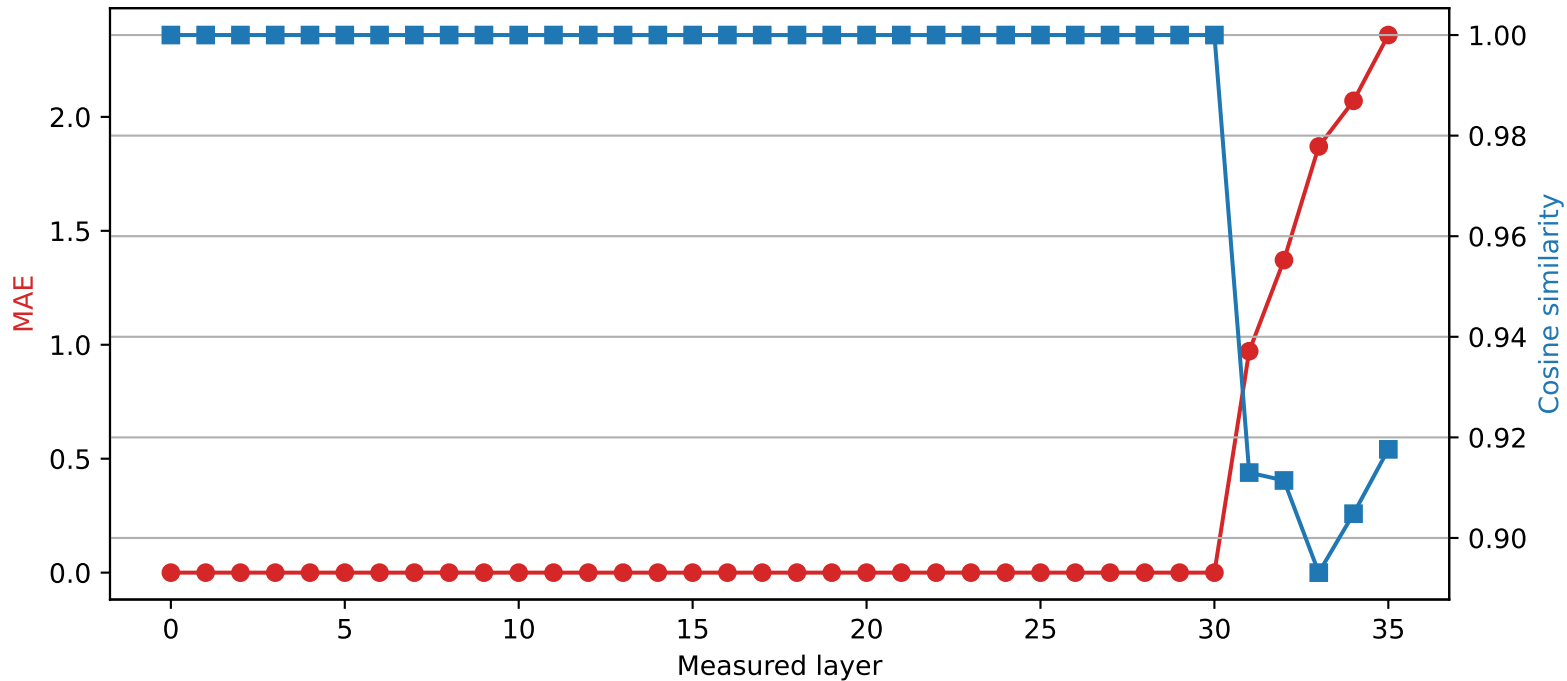
Qwen2.5-3B | Quantized layer 30 | float32 \rightarrow int8
