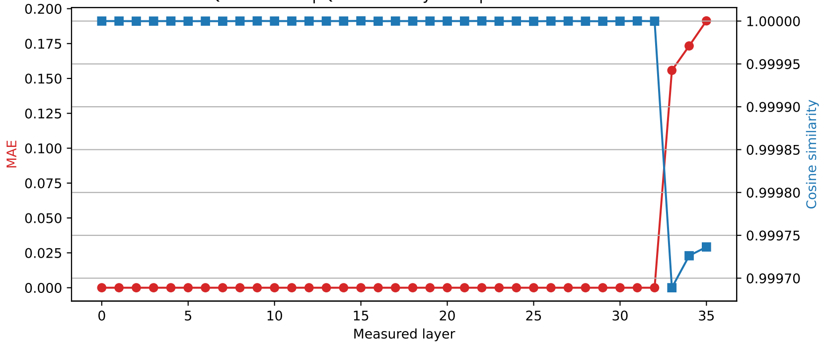
Qwen2.5-3B | Quantized layer 32 | float32 → int8
