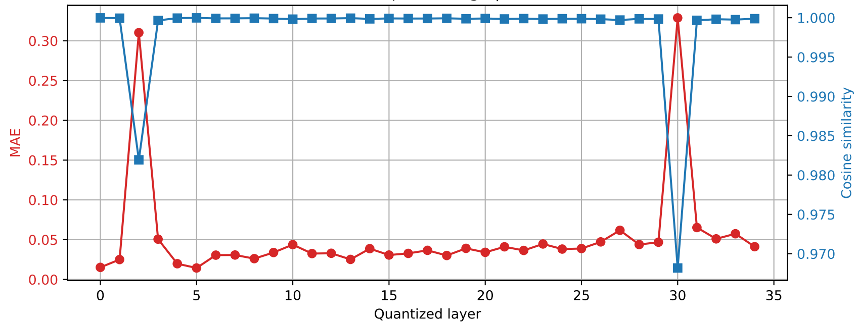
Qwen2.5-3B | Prompt 1 Final RMSNorm output damage | float32 → int8
