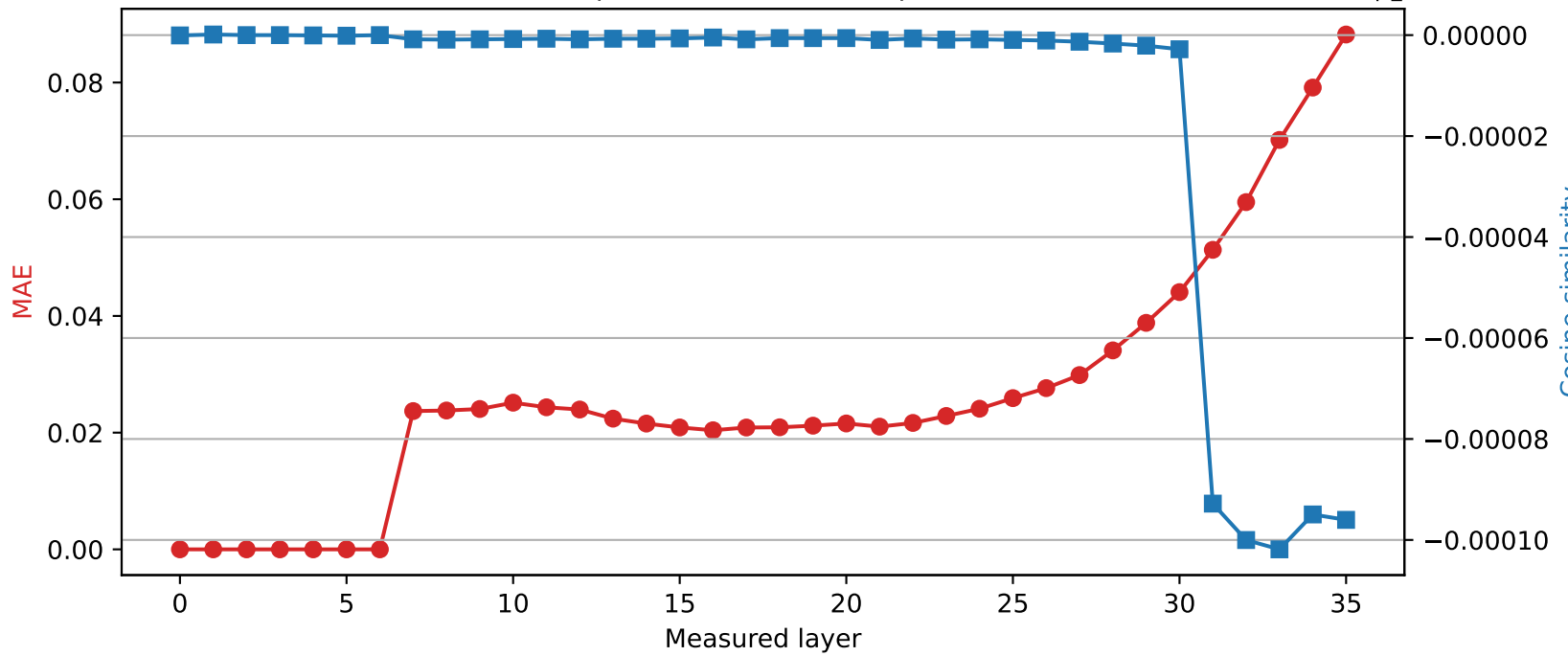
Qwen2.5-3B | Quantized layer 6 | float32 → int8
