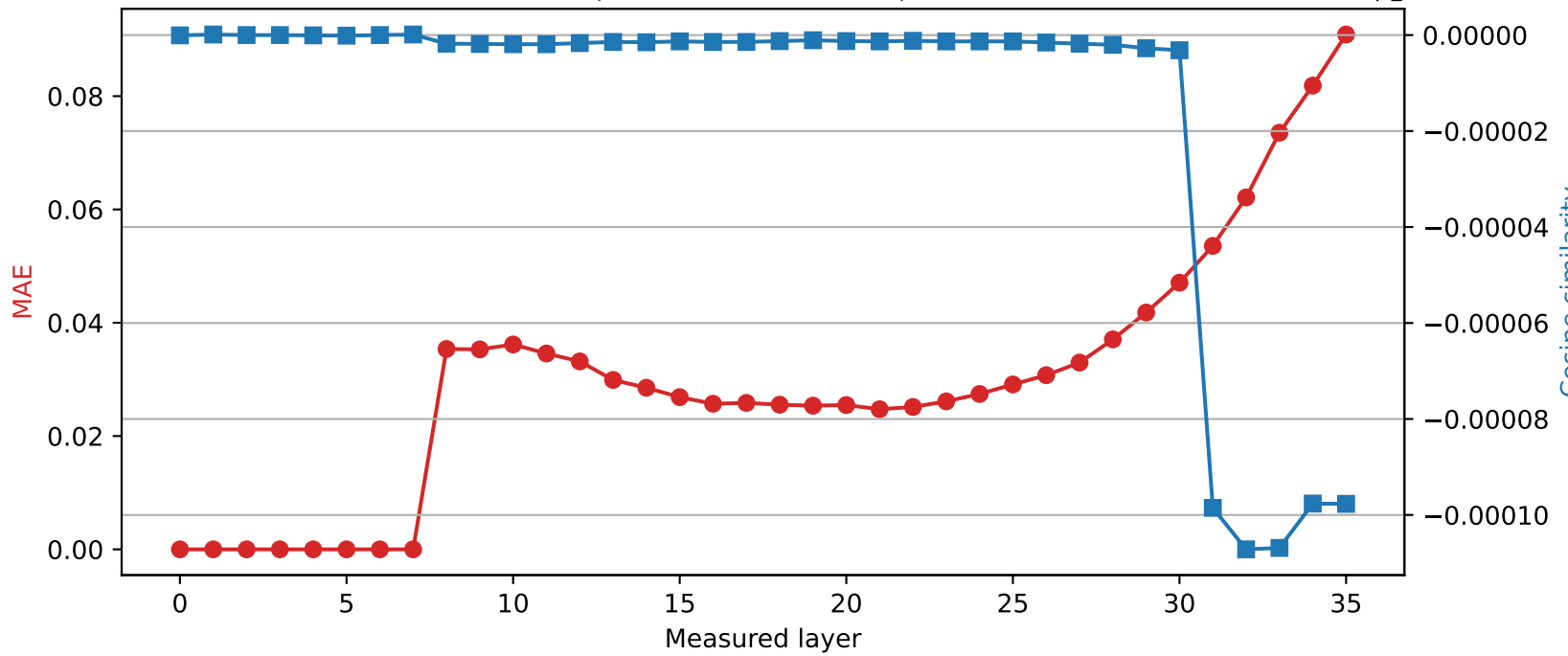
Qwen2.5-3B | Quantized layer 7 | float32 \rightarrow int8
