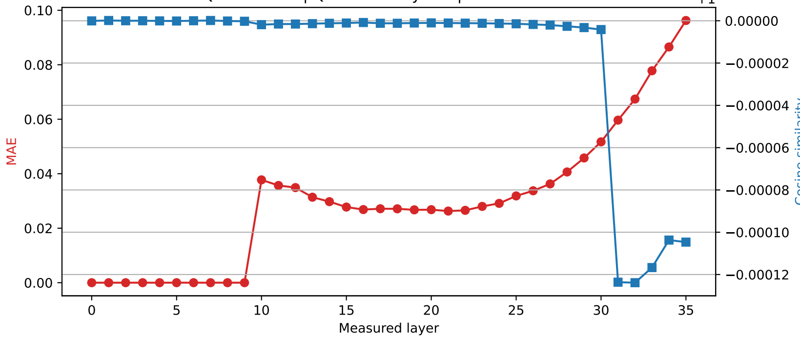
Qwen2.5-3B | Quantized layer 9 | float32 \rightarrow int8
