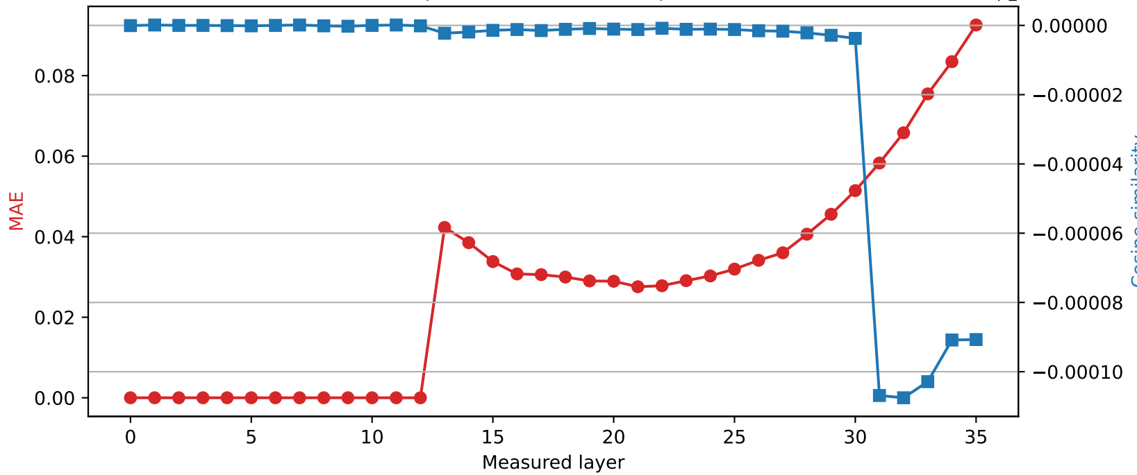
Qwen2.5-3B | Quantized layer 12 | float32 → int8
