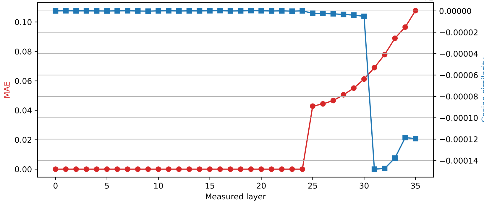
Qwen2.5-3B | Quantized layer 24 | float32 → int8
