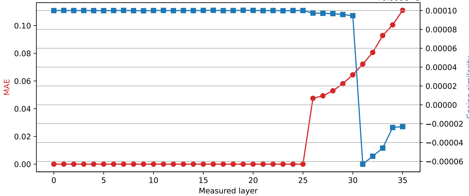
Qwen2.5-3B | Quantized layer 25 | float32 → int8
