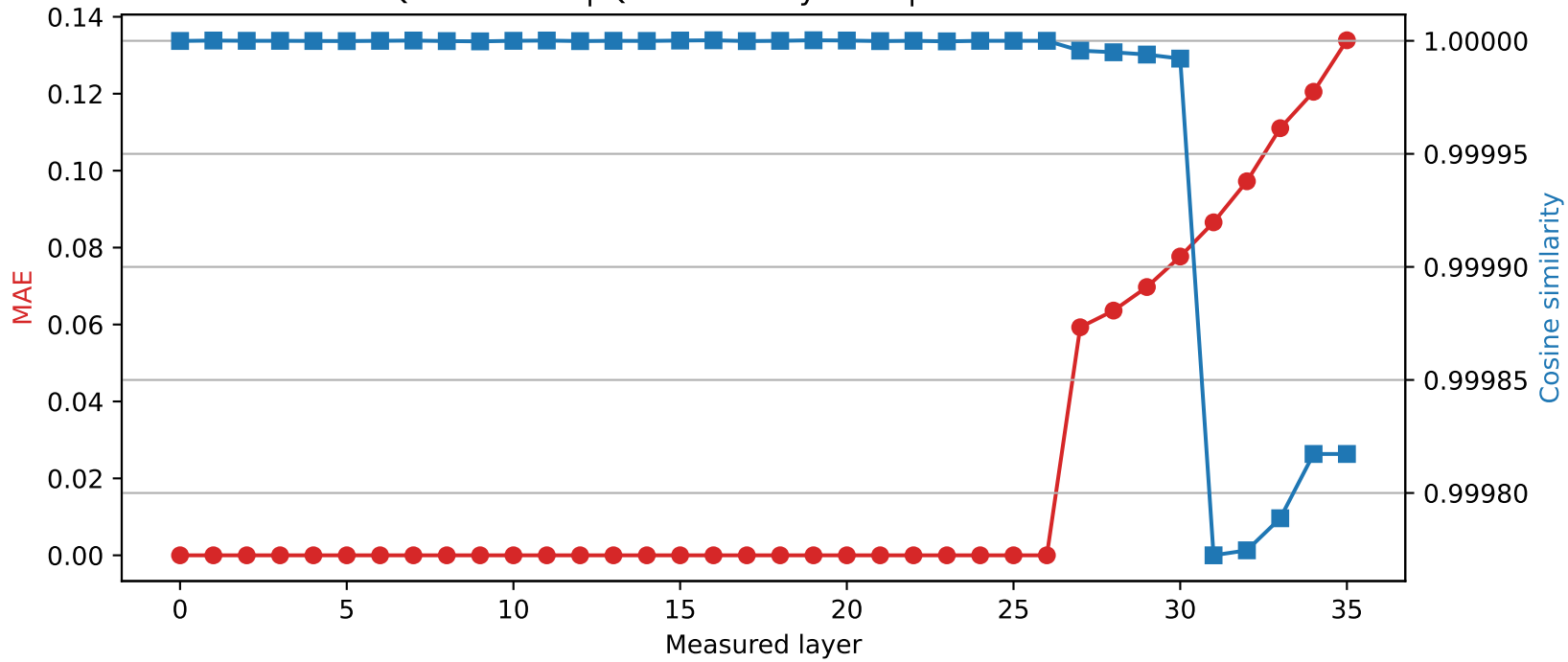
Qwen2.5-3B | Quantized layer 26 | float32 \rightarrow int8
