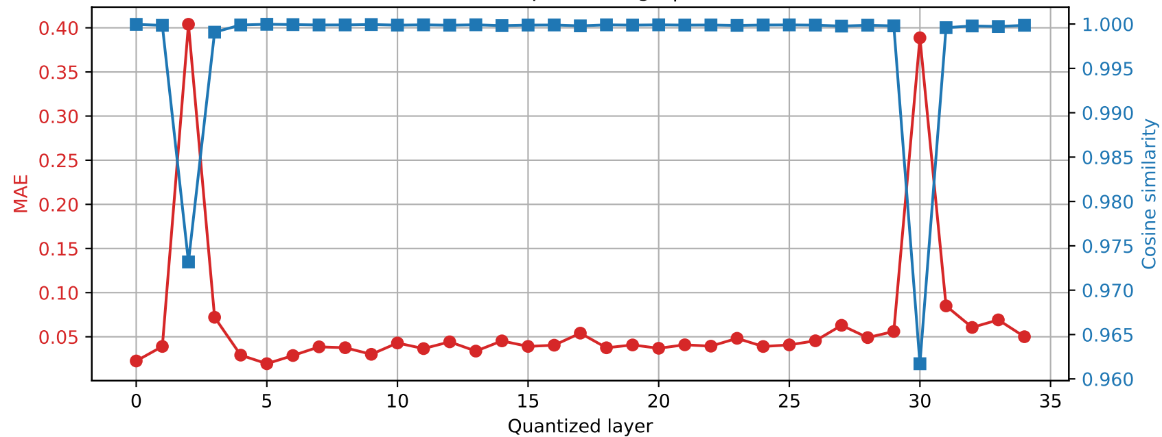
Qwen2.5-3B | Prompt 2 Final RMSNorm output damage | float32 \rightarrow int8
