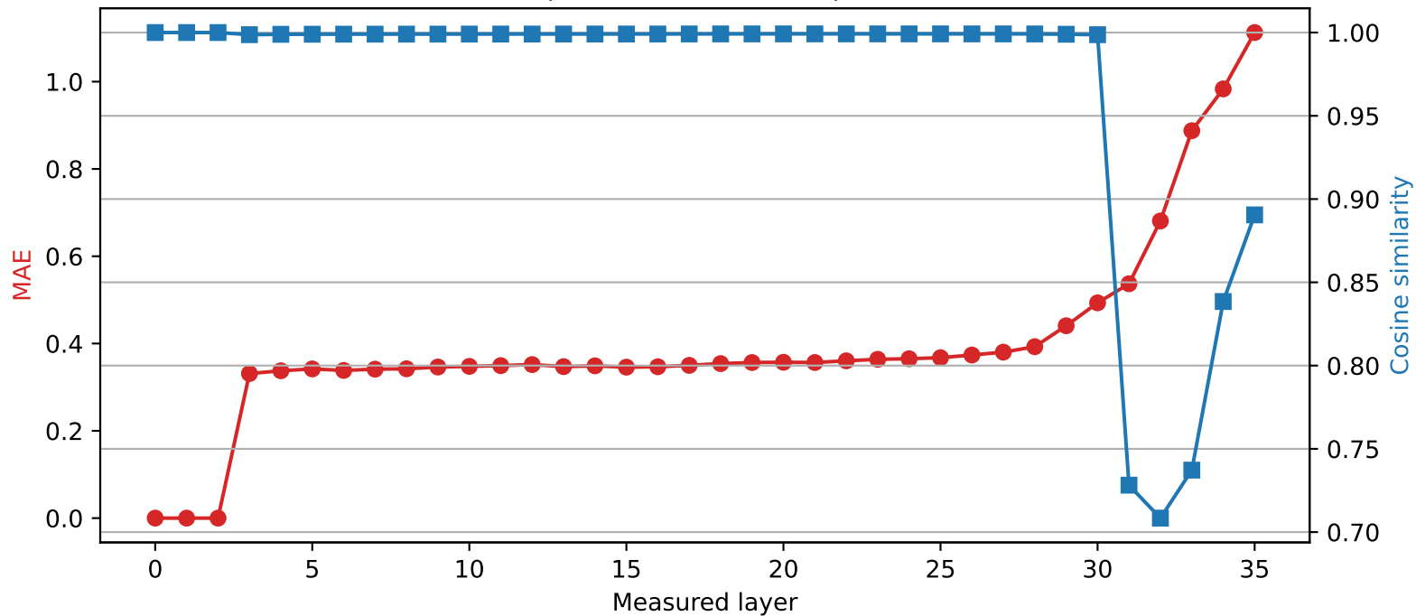
Qwen2.5-3B | Quantized layer 2 | float32 \rightarrow int8
