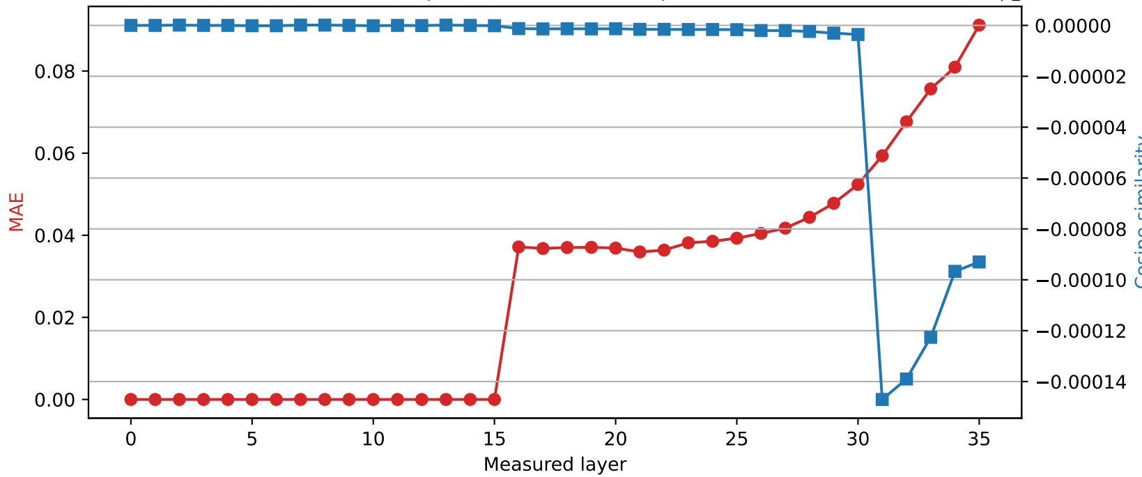
Qwen2.5-3B | Quantized layer 15 | float32 → int8
