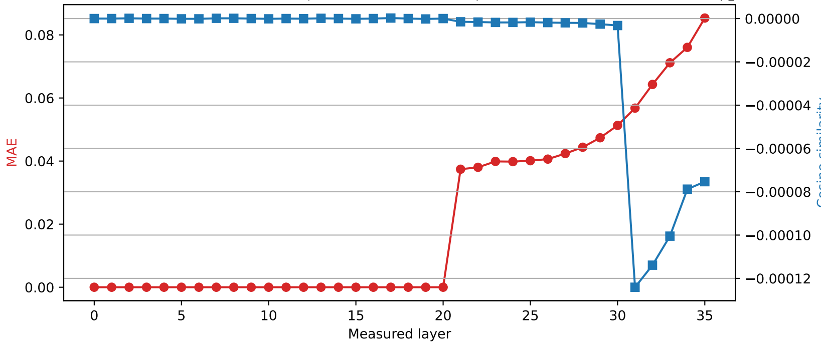
Qwen2.5-3B | Quantized layer 20 | float32 → int8
