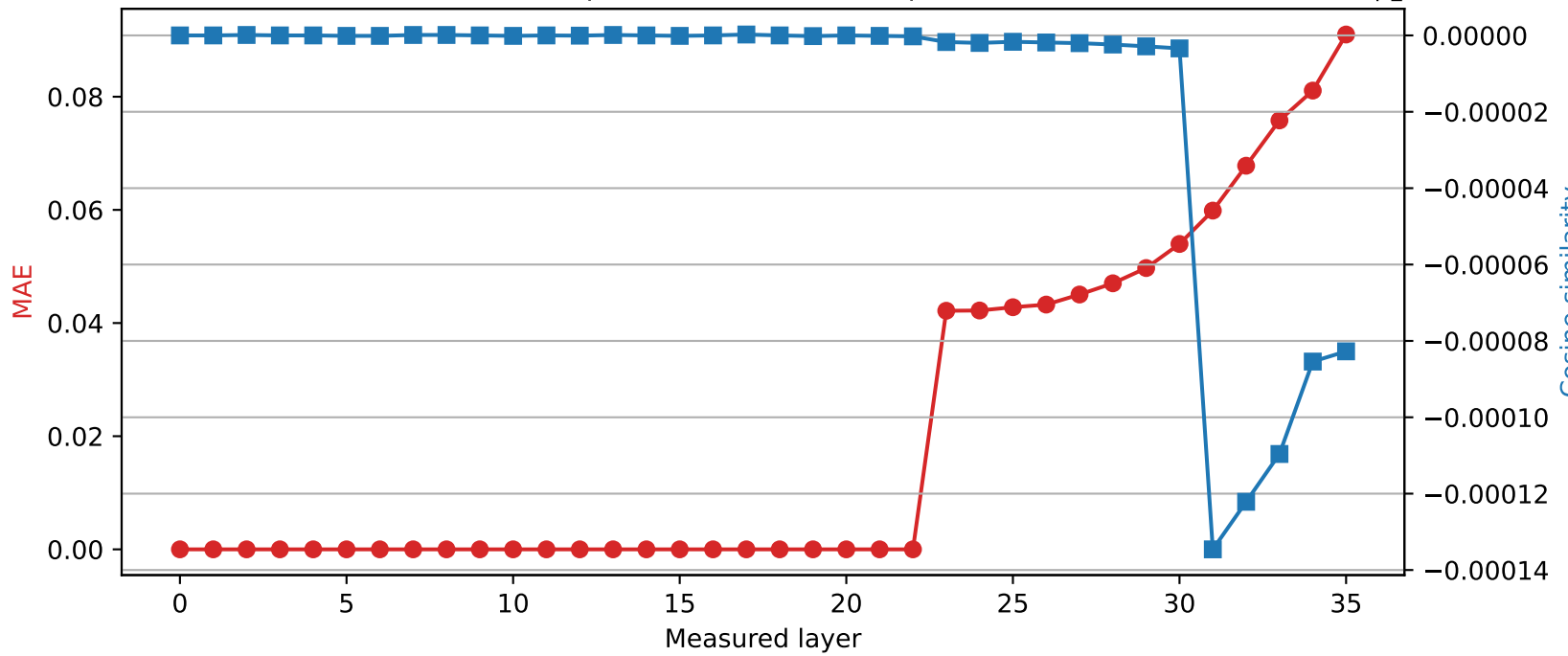
Qwen2.5-3B | Quantized layer 22 | float32 → int8
