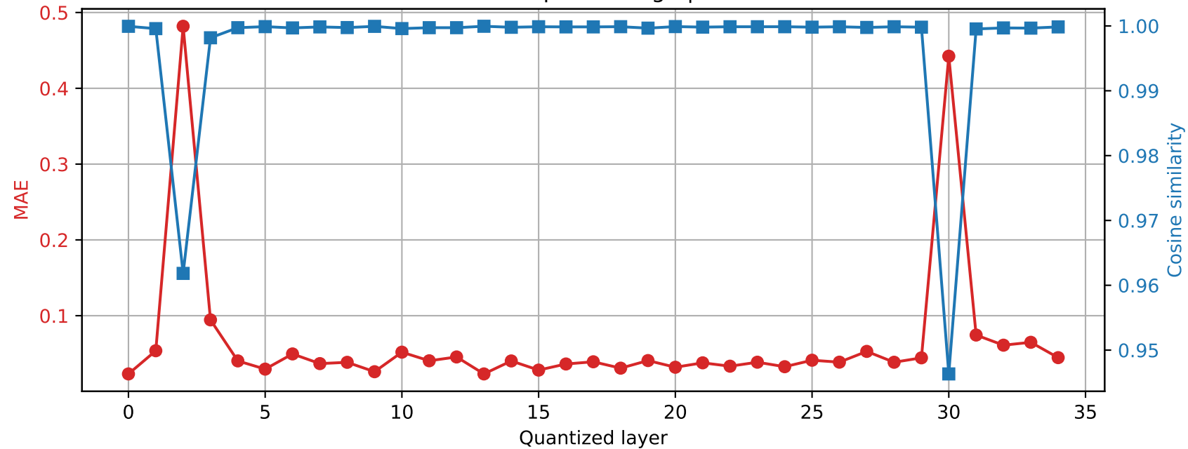
Qwen2.5-3B | Prompt 3 Final RMSNorm output damage | float32 \rightarrow int8
