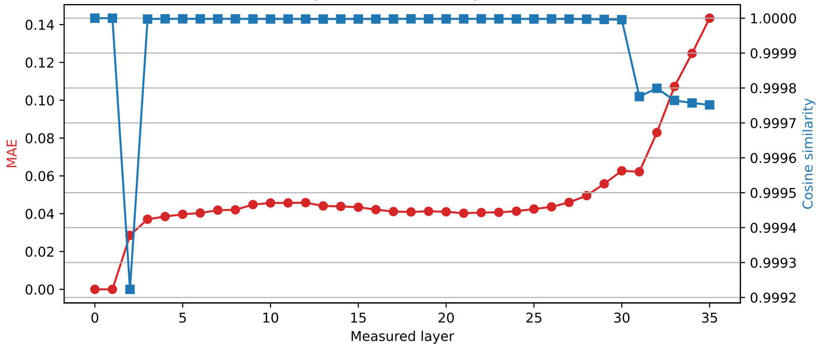
Qwen2.5-3B | Quantized layer 1 | float32 → int8
