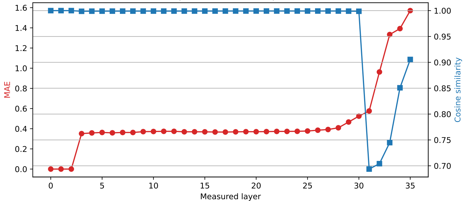
Qwen2.5-3B | Quantized layer 2 | float32 → int8
