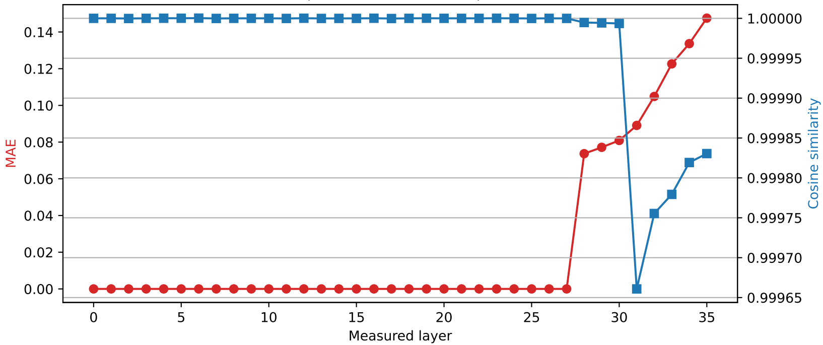
Qwen2.5-3B | Quantized layer 27 | float32 → int8
