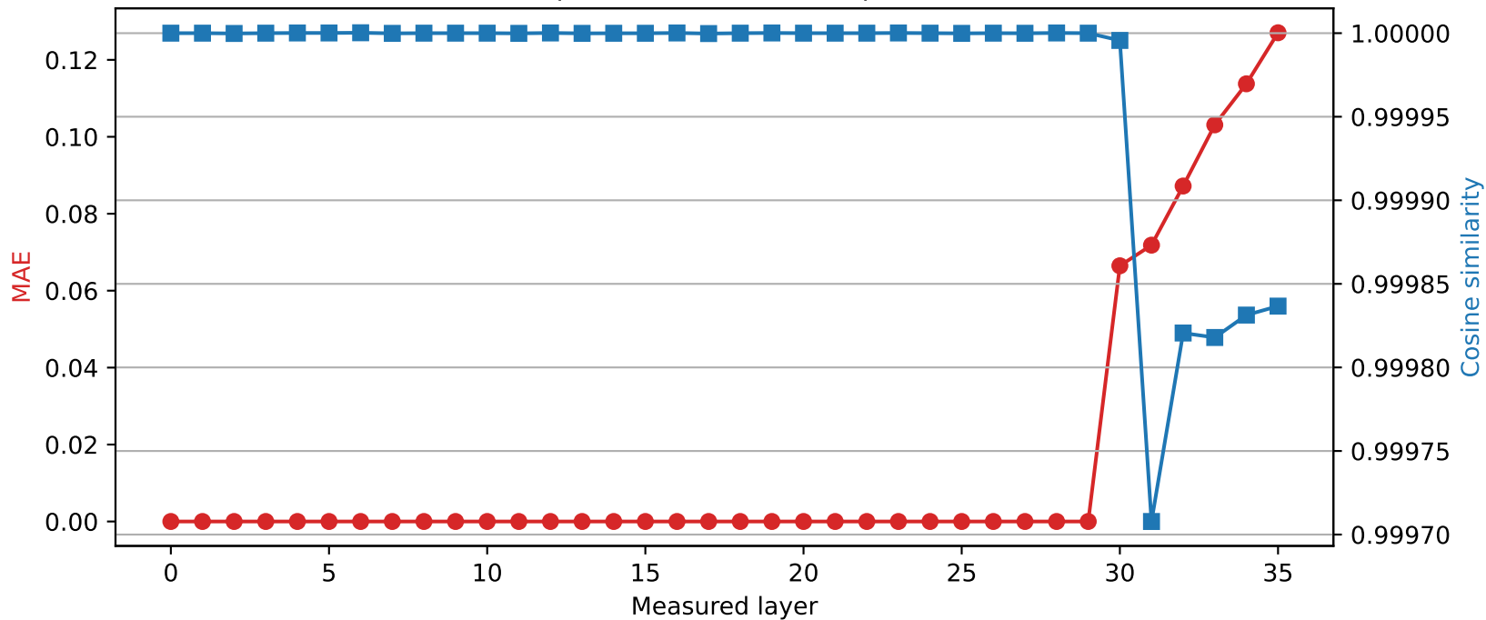
Qwen2.5-3B | Quantized layer 29 | float32 \rightarrow int8
