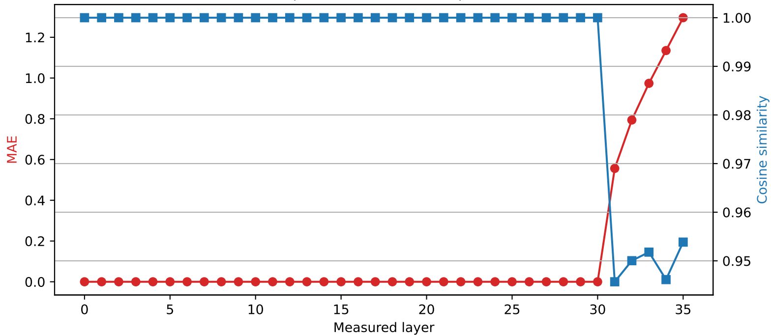
Qwen2.5-3B | Quantized layer 30 | float32 → int8
