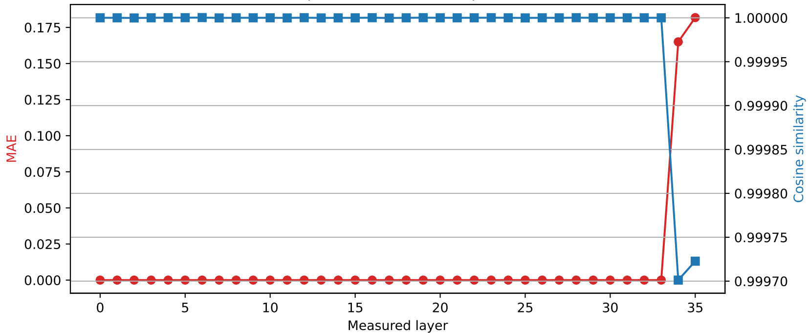
Qwen2.5-3B | Quantized layer 33 | float32 \rightarrow int8
