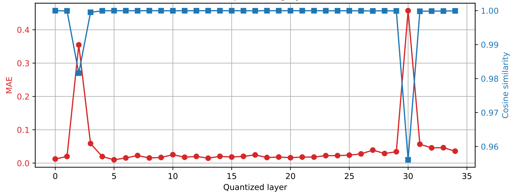
Qwen2.5-3B | Prompt 4 Final RMSNorm output damage | float32 → int8
