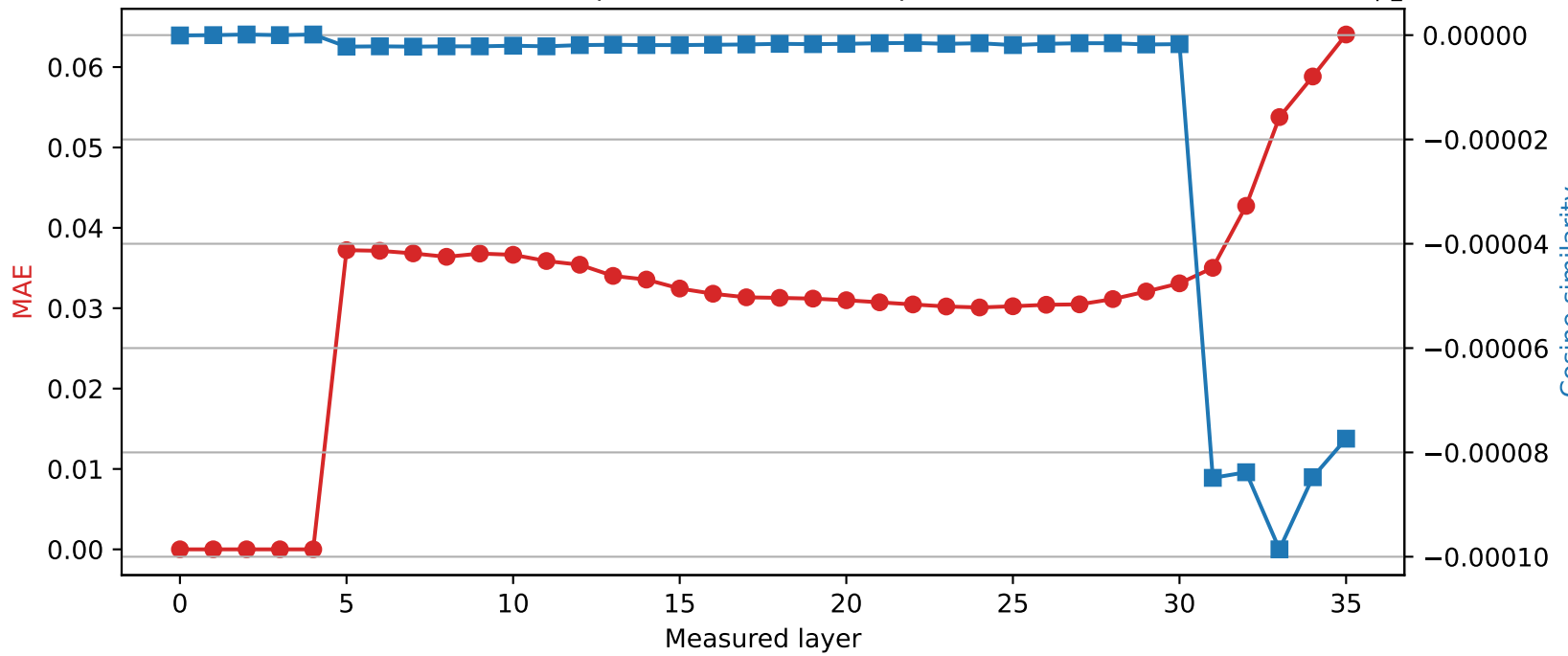
Qwen2.5-3B | Quantized layer 4 | float32 \rightarrow int8
