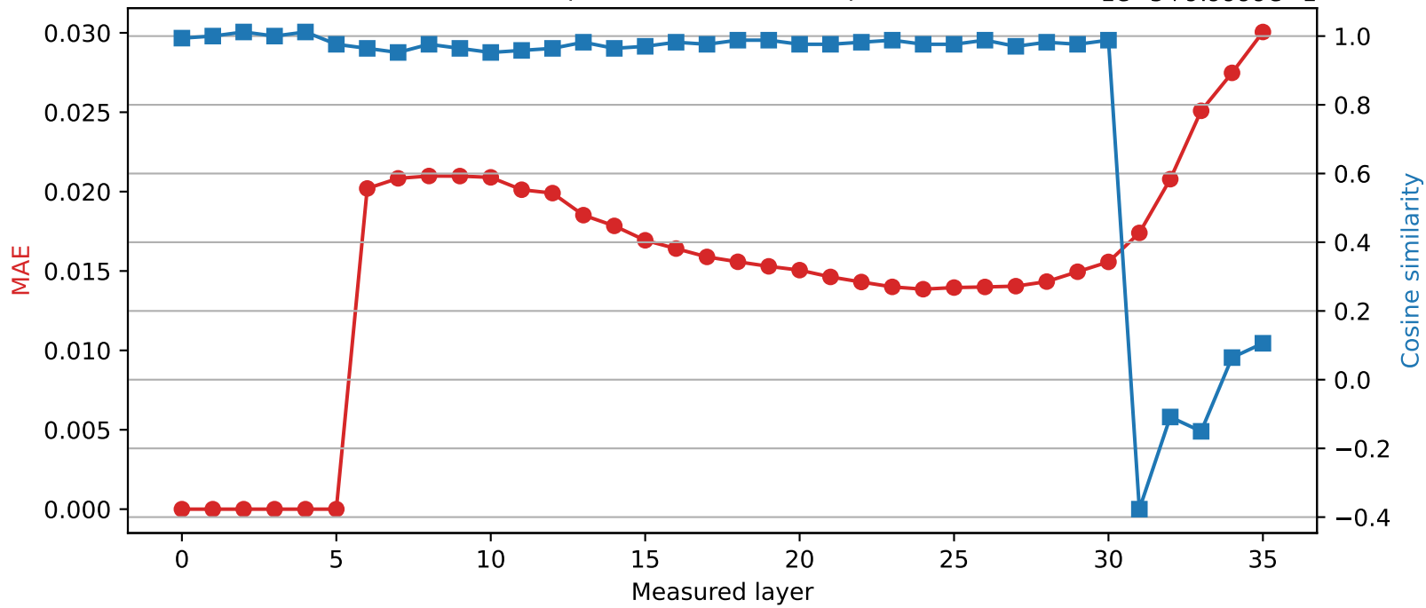
Qwen2.5-3B | Quantized layer 5 | float32 \rightarrow int8
