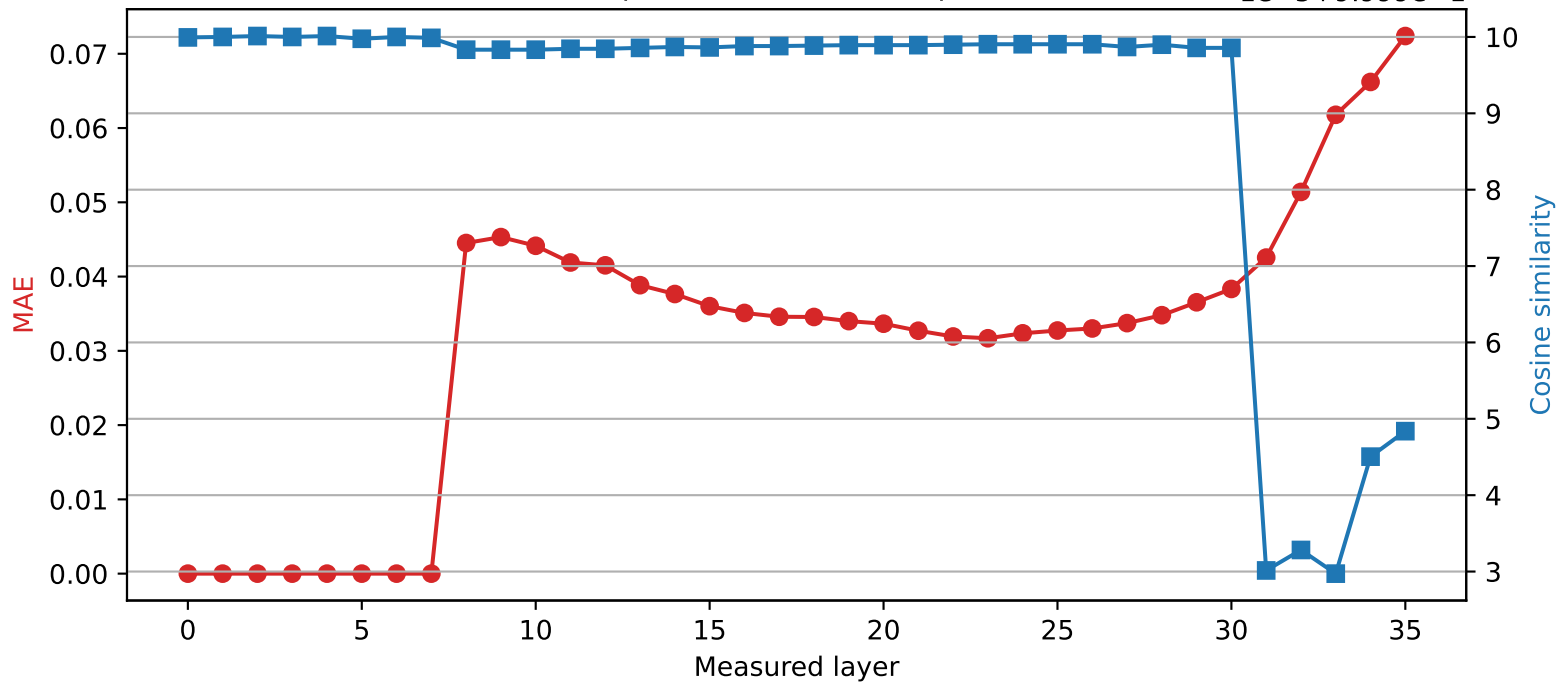
Qwen2.5-3B | Quantized layer 7 | float32 → int8
