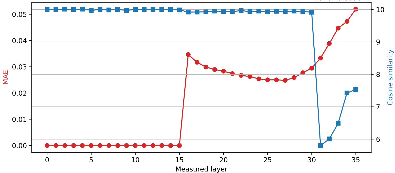
Qwen2.5-3B | Quantized layer 15 | float32 → int8
