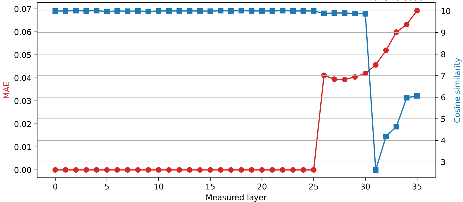
Qwen2.5-3B | Quantized layer 25 | float32 → int8
